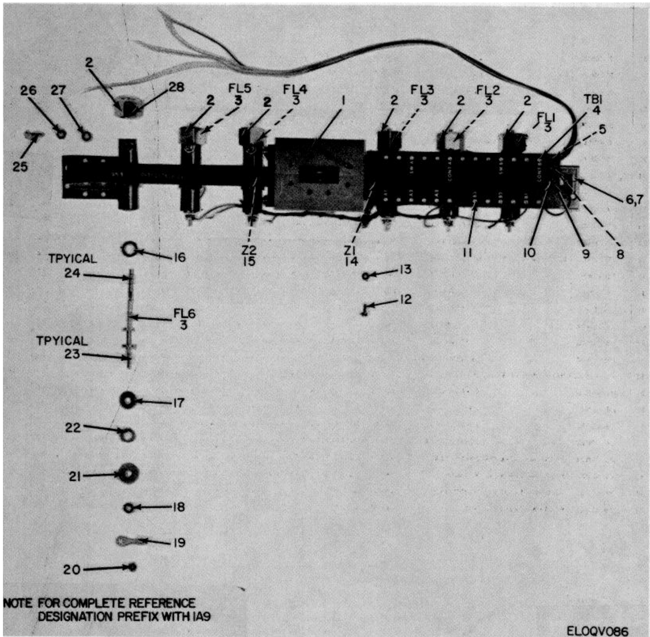
Figure 51. Waveguide Assembly, Transmitter (1A9).
