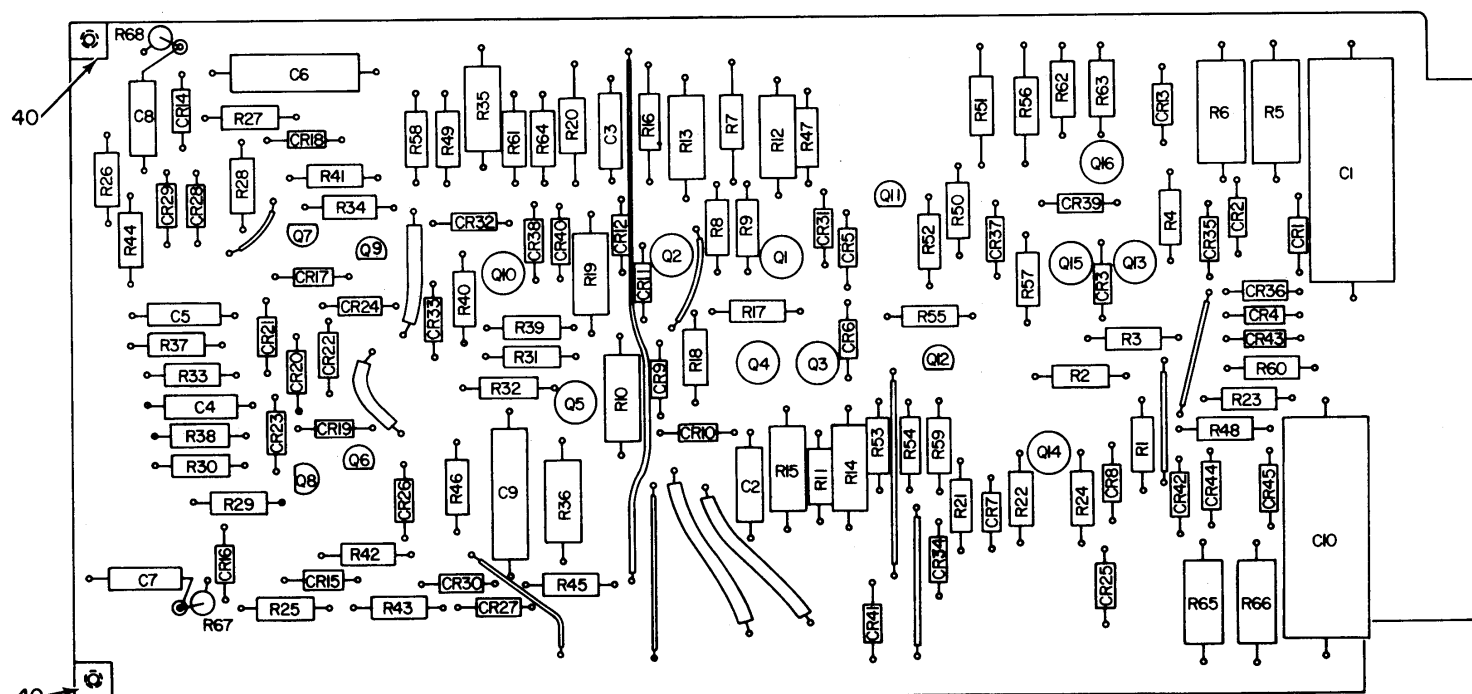
BOARD VIEW
