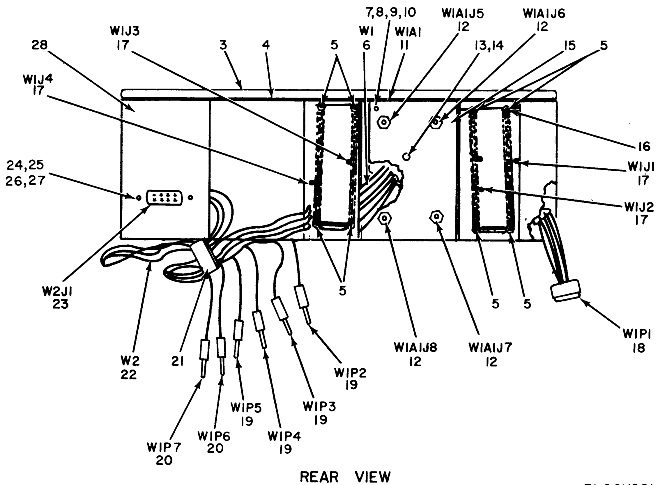
Figure 55. Pre-emphasis and De-emphasis Assembly (1A10) (Sheet 2 of 2).
